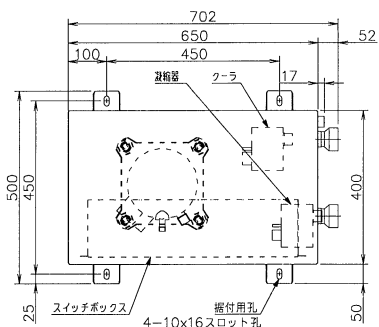
RUW-P1501, P2241, P3001
