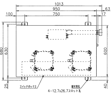
RUW-P4501(V), P6001(V)
