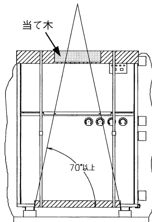
RUW-P4501, P6001
