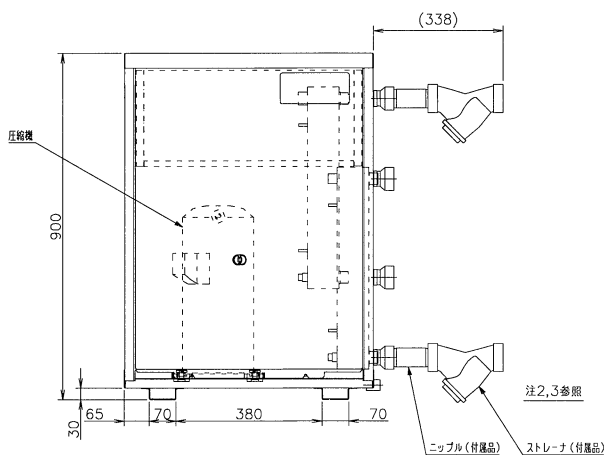
RUW-P4501(V), P6001(V)
