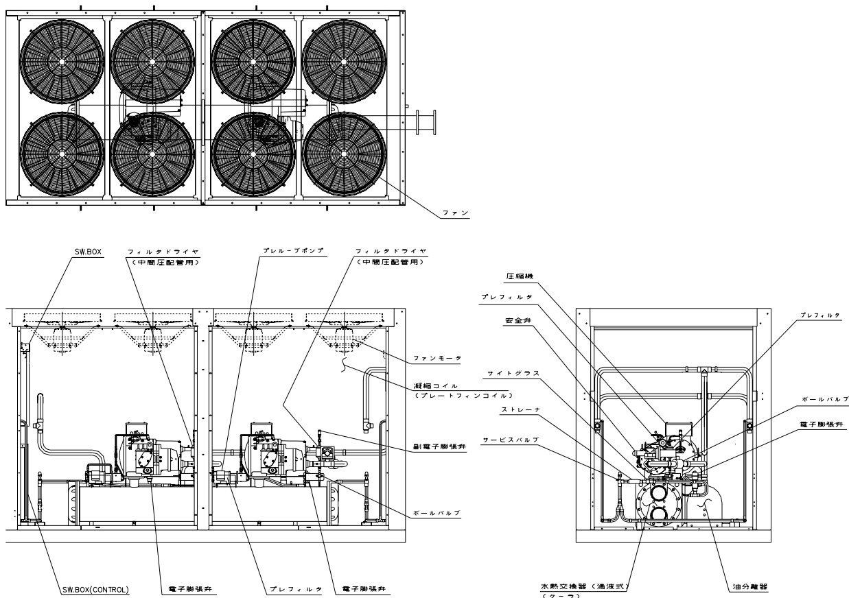
RUA-SB35505-B, SB42505-A/B
