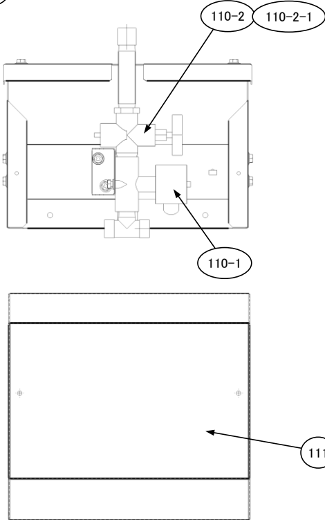
110 DETAIL (High-EER type only)
