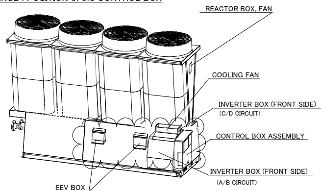
100 CONTROL BOX ASSEMBLY
