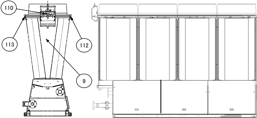
112 DETAIL (PIPE ASSEMBLY, HEAT EXCHANGER WATER SPRAY SYSTEM (LEFT))
